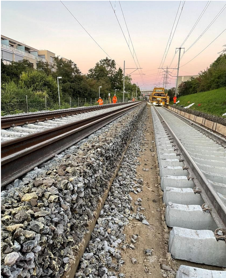
View of the uncovered bonding ballast
