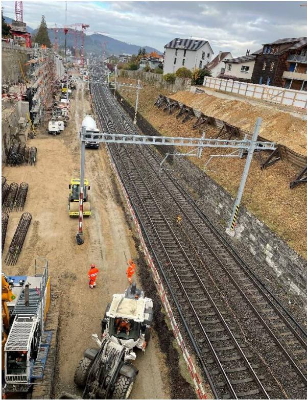
View of the construction site and the track to be bonded
